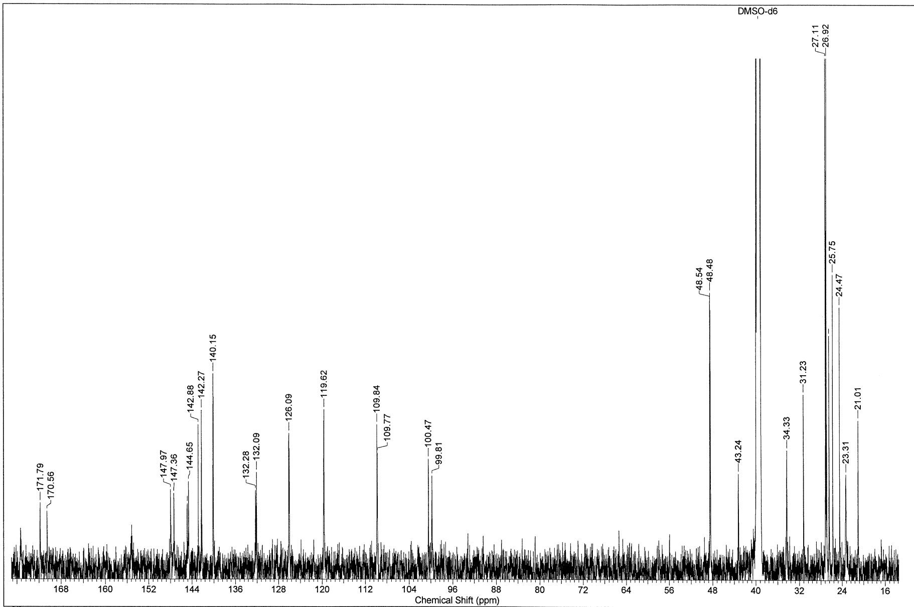
^{13}\text{C} NMR (DMSO- d_6 , 150 MHz)
